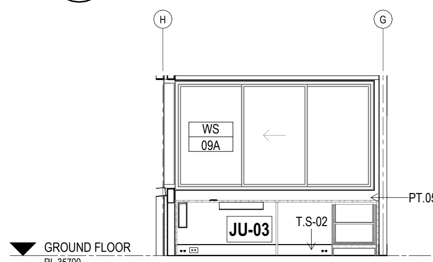
O ELEVATION OFFICIALS ROOM Scale: 1: 50
