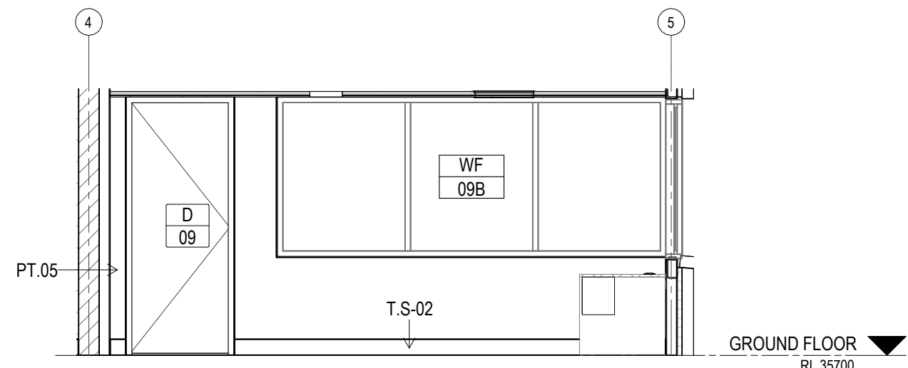
N ELEVATION OFFICIALS ROOM Scale: 1: 50
