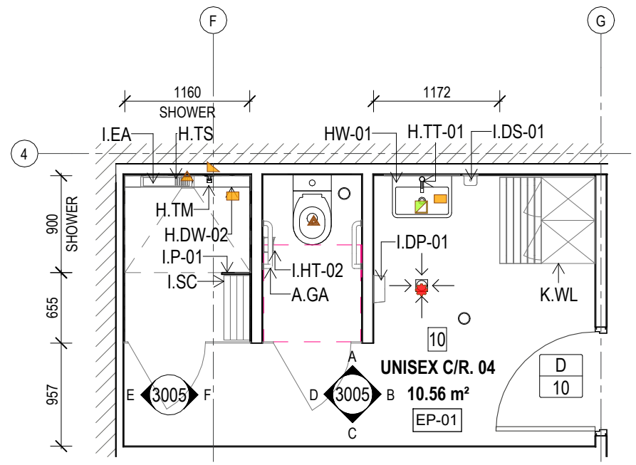
1 PLAN ROOM LAYOUT - UNISEX C/R.04 Scale: 1: 50
