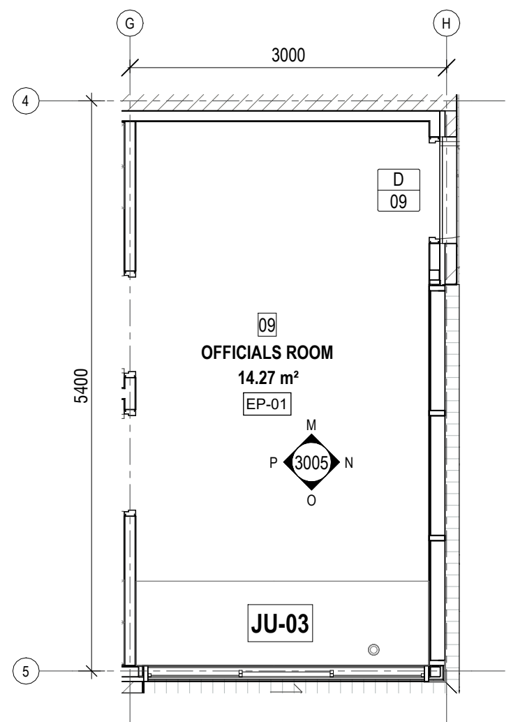
5 PLAN ROOM LAYOUT - OFFICIALS ROOM Scale: 1: 50
