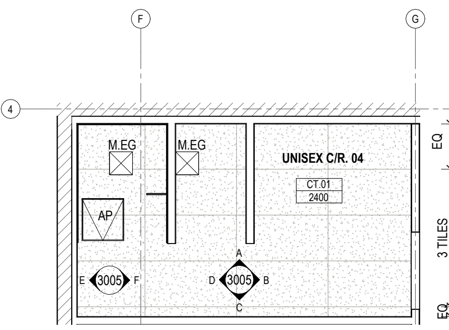
2 REFLECTED CEILING PLAN UNISEX C/R.04 Scale: 1: 50
