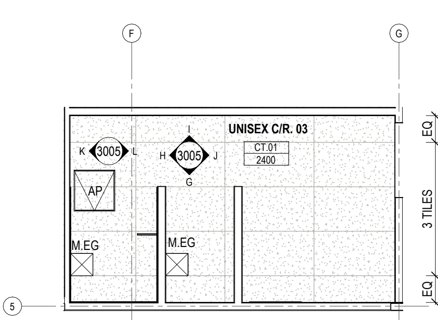
4 REFLECTED CEILING PLAN UNISEX C/R.03 Scale: 1: 50
