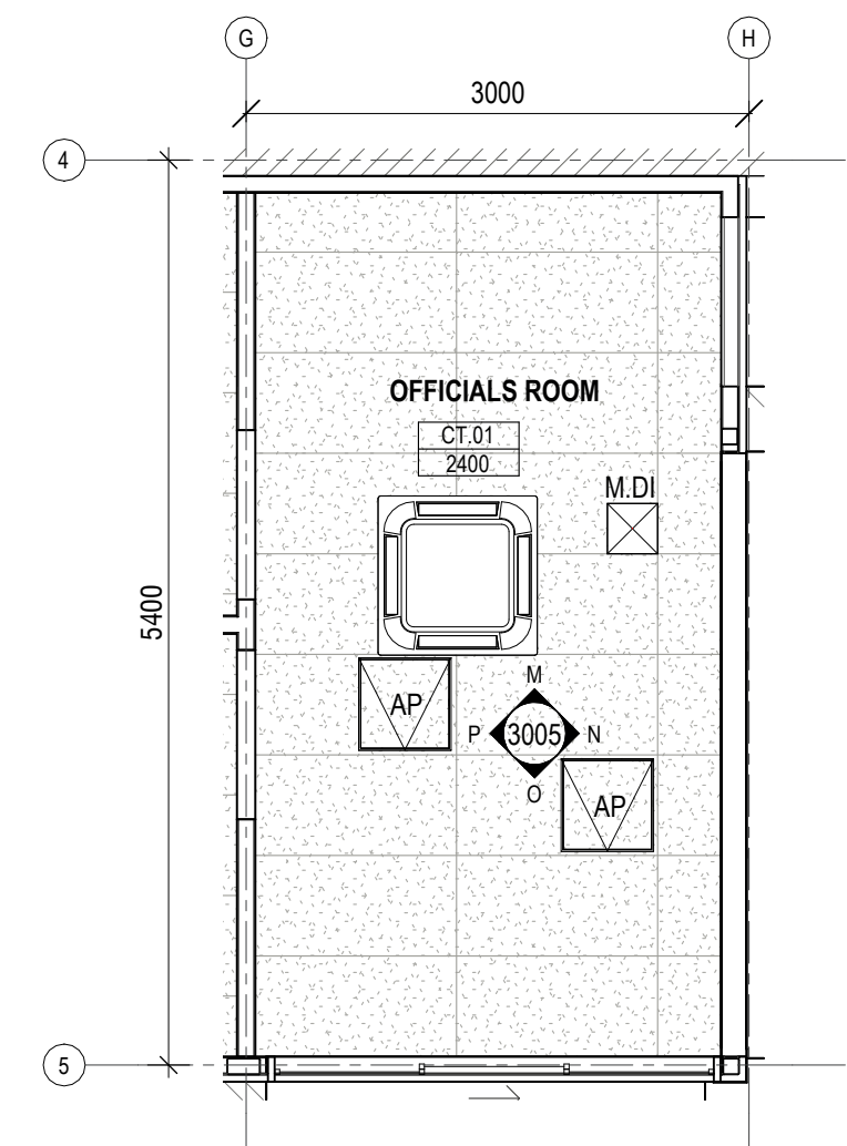
6 REFLECTED CEILING PLAN OFFICIALS ROOM Scale: 1: 50
